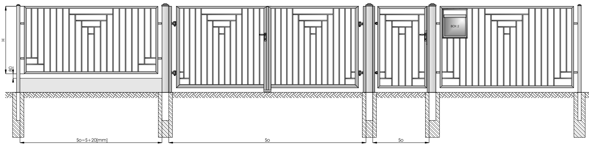
System Lux RYS. L10.55D
